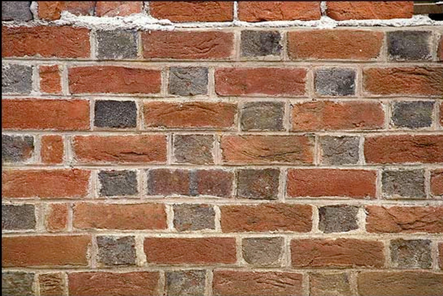
Staggered Rows of Bricks that are Laid End to Side (Colonial Williamsburg)
