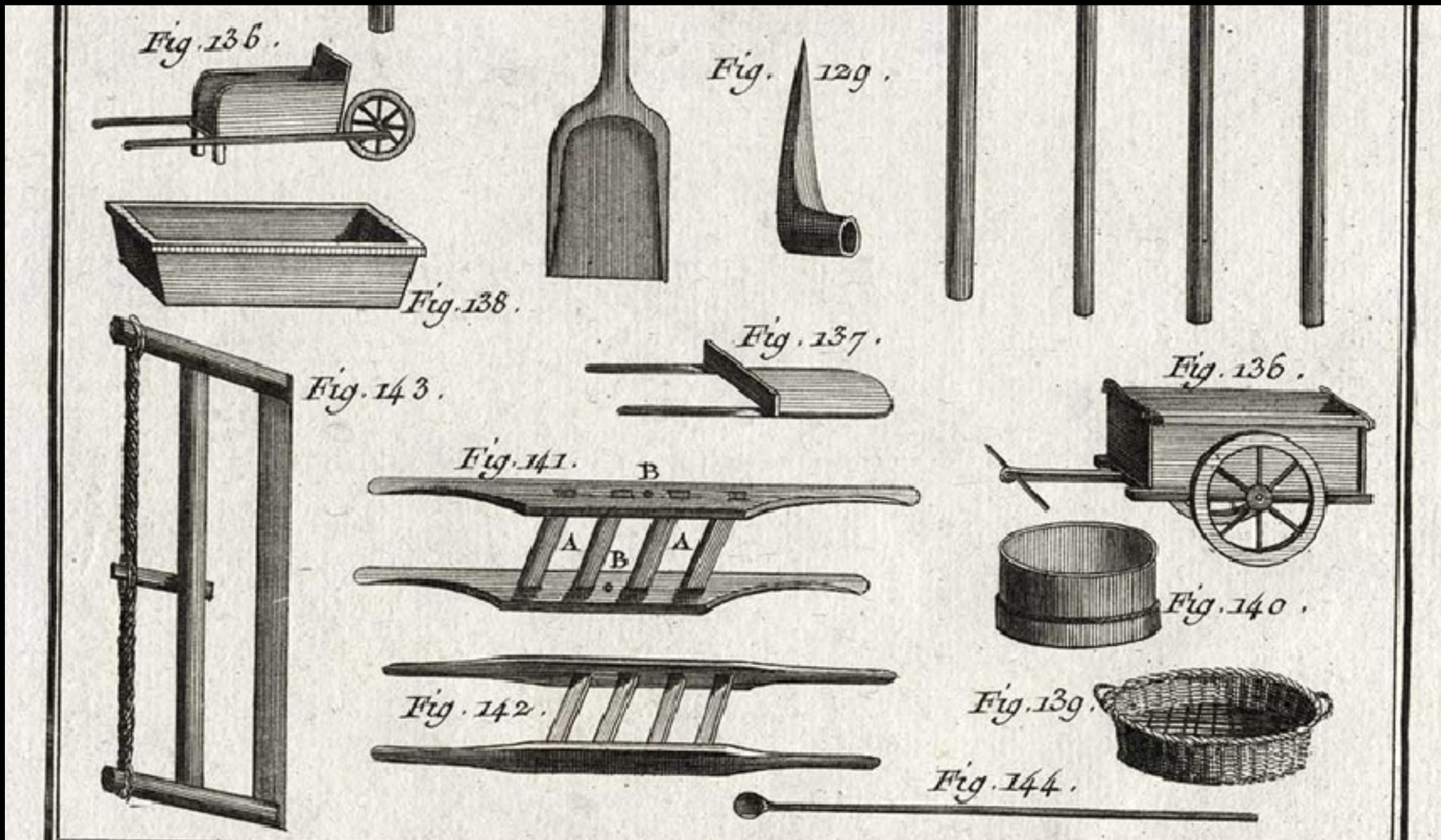
“Architecture, Maçonnerie” The Encyclopedia of Diderot & d'Alembert 1763
