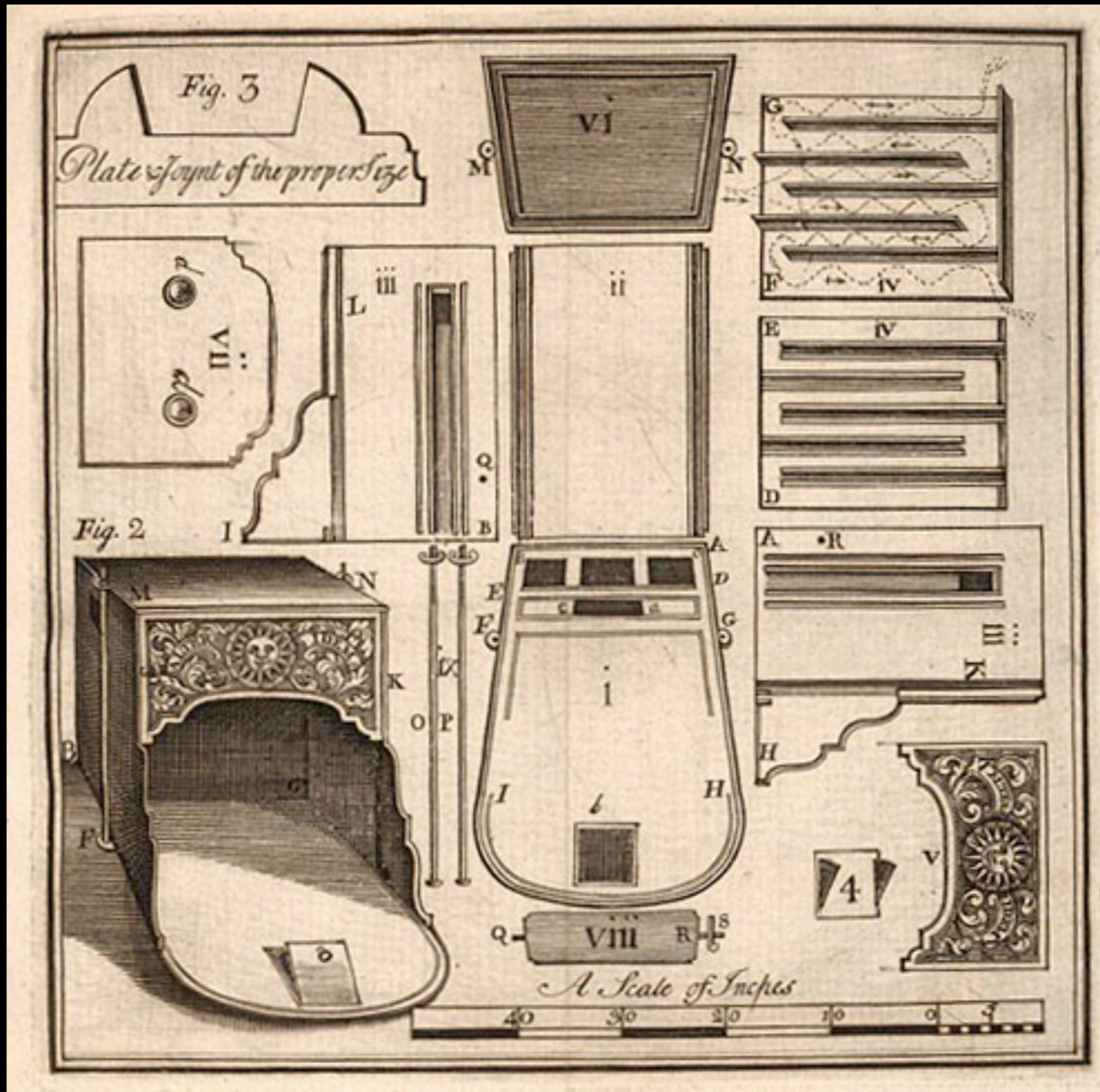
Illustration of Benjamin Franklin's Pennsylvania Stove, Published in "An Account of the New Invented Pennsylvanian Fire-Places" Philadelphia, Pennsylvania 1744
