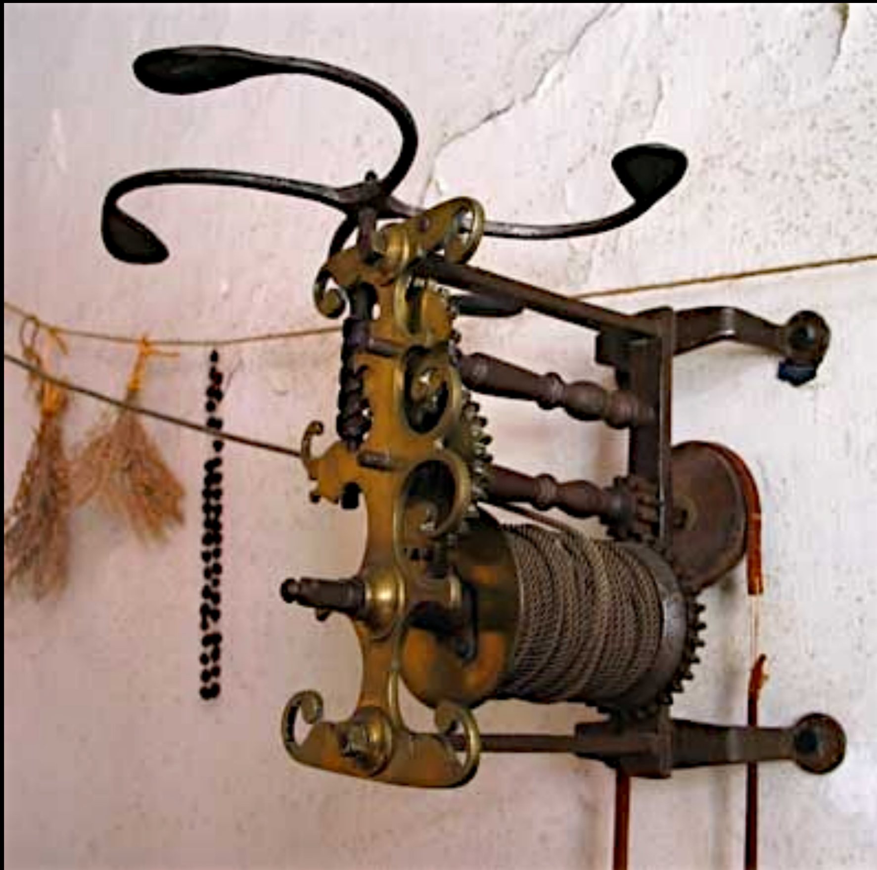
English Spitjack 18th Century (Webb Deane Stevens Museum, Connecticut)
