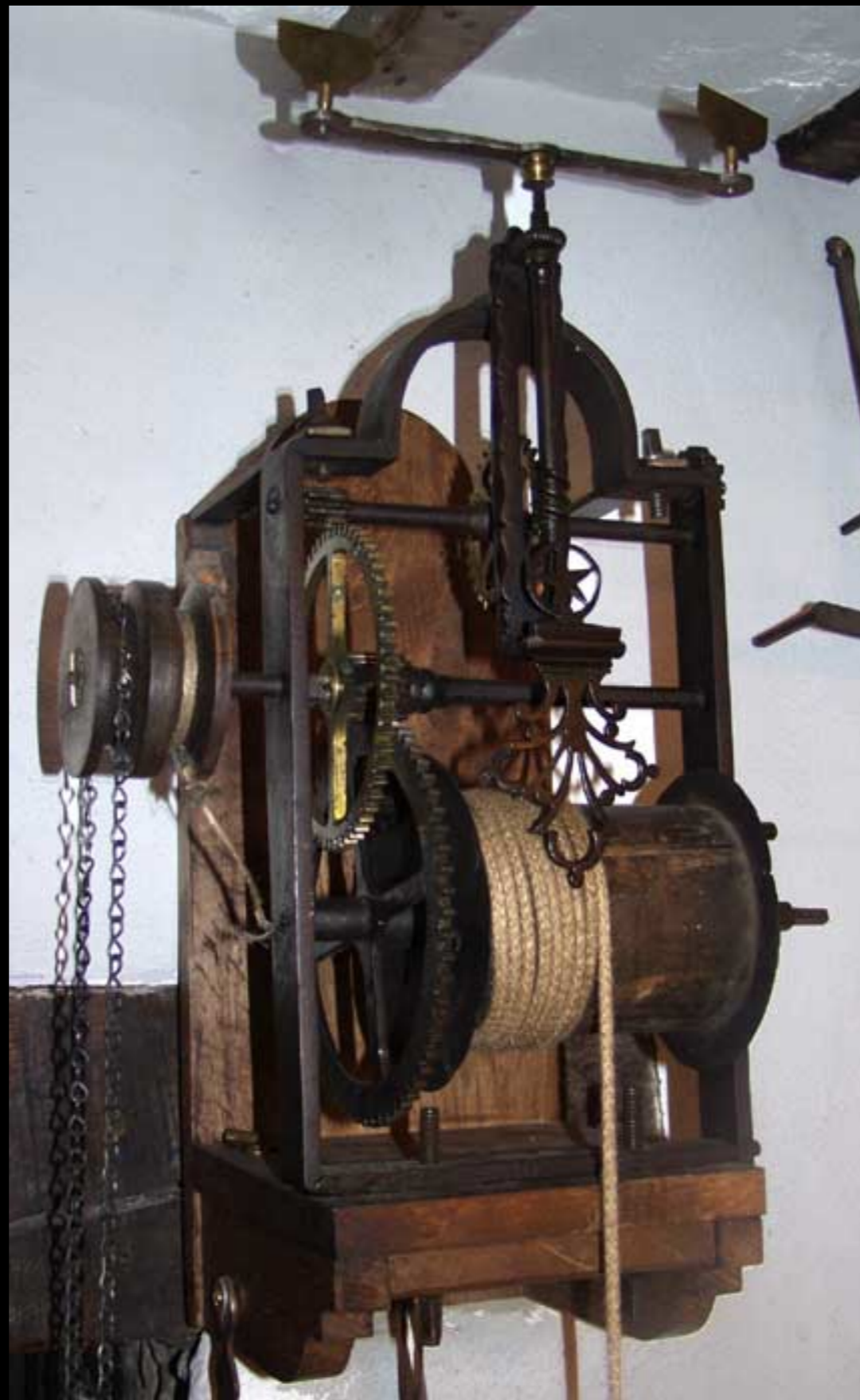
Weight Driven Spitjack Early 18th Century (Wreay Farm)
