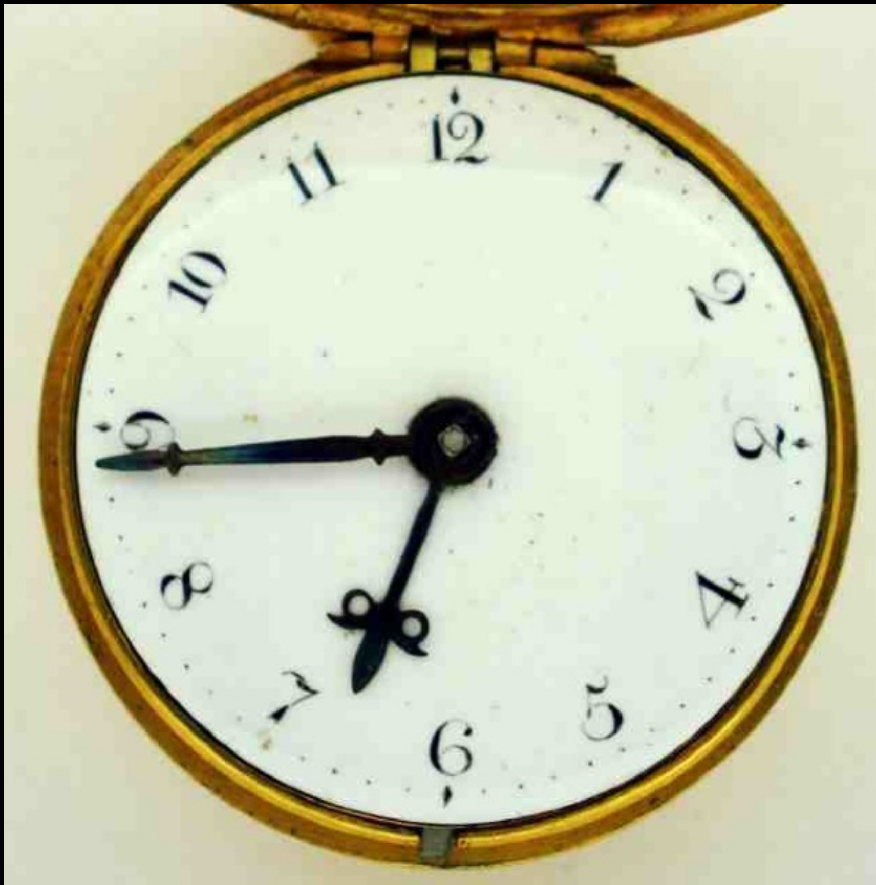
English Gilt & Shell Pair Cased Watch with Verge Movement by George Graham of London c. 1747 (Cogs & Pieces, Antique Pocket Watches)
