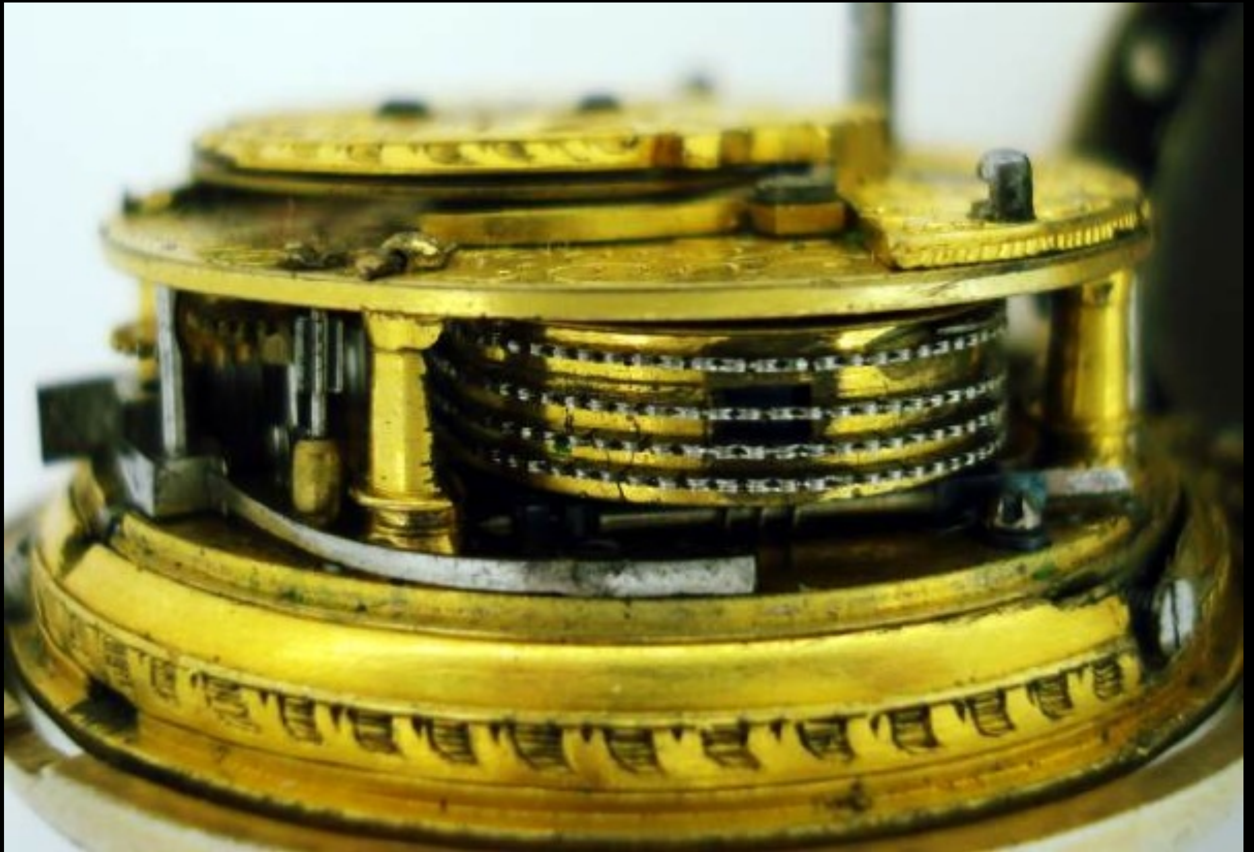
English Gilt Pair Cased Watch with Verge Movement, Quarter Repeat by Andrew Dunlop of London c. 1720 (Cogs & Pieces, Antique Pocket Watches)
