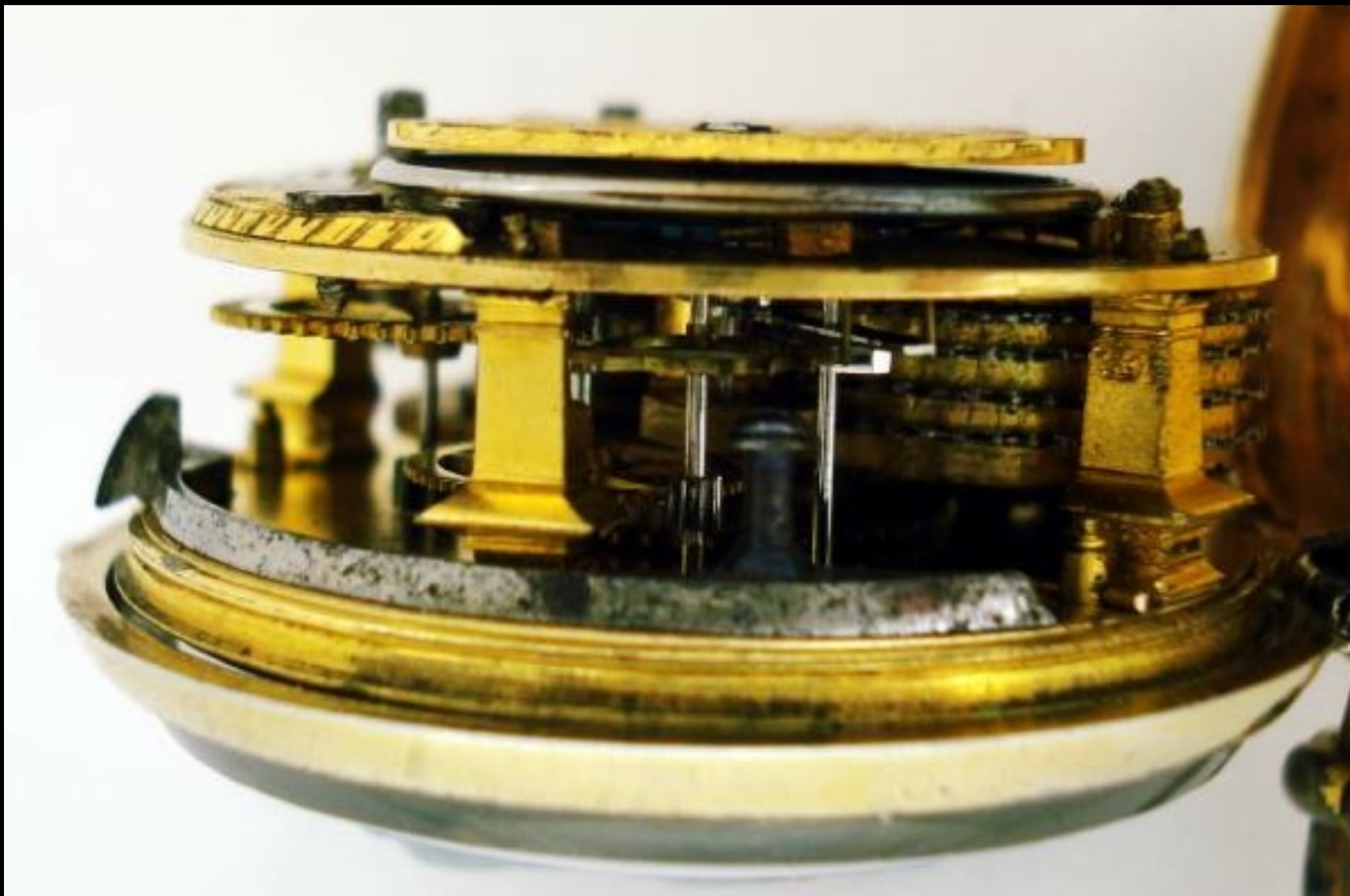
English Silver Gilt Repousse Pair Cased Watch with Lever Movement by Ritter of London c. 1740 (Cogs & Pieces, Antique Pocket Watches)
