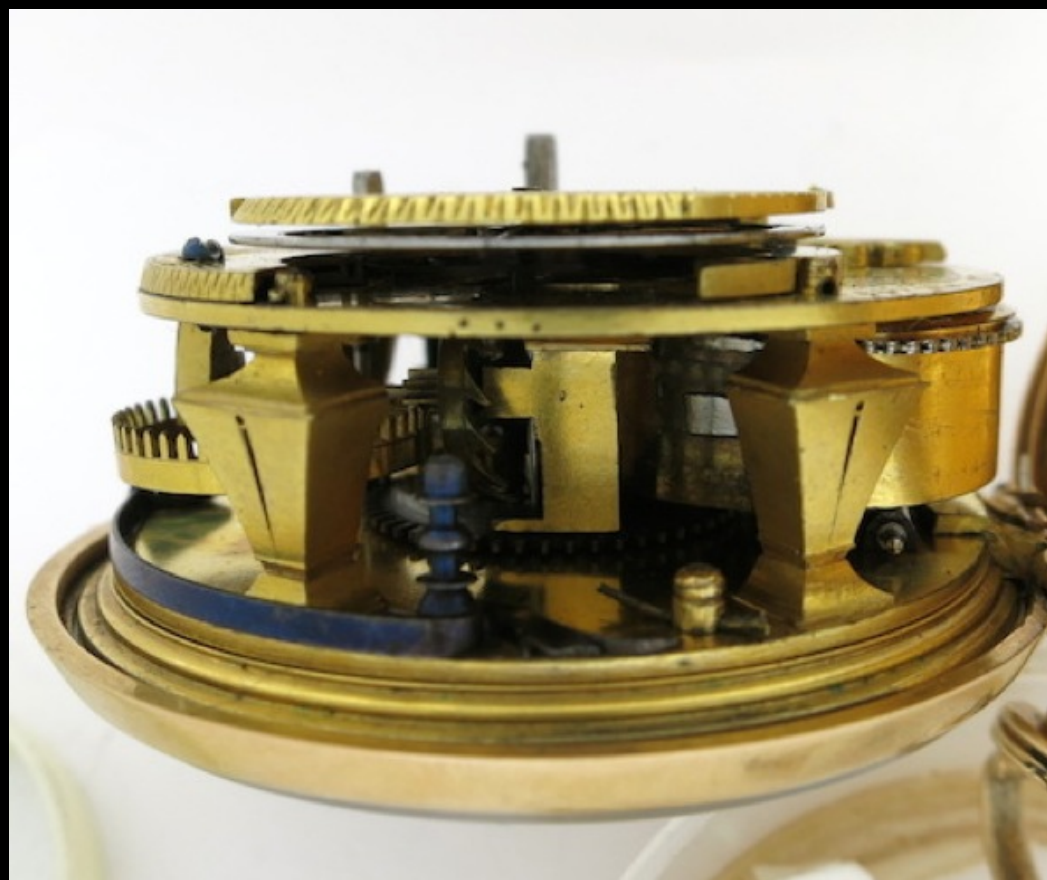
English Gold & Gilt Pair Cased Watch with Verge Movement by Broukner Watts of London c. 1710 (Cogs & Pieces, Antique Pocket Watches)
