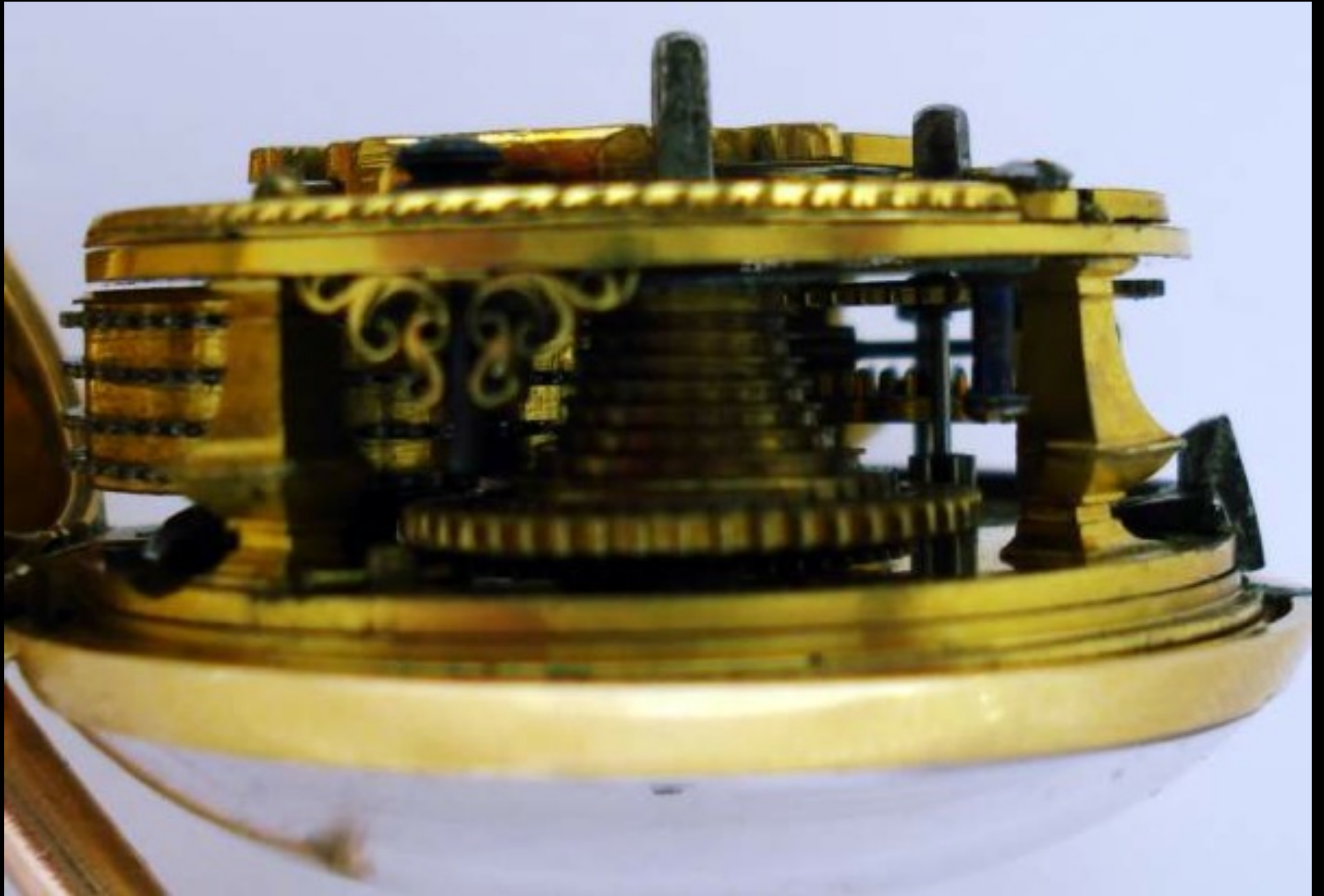
English Gold Repousse Pair Cased Watch with Verge Movement by John Weldon of London 1728 (Cogs & Pieces, Antique Pocket Watches)
