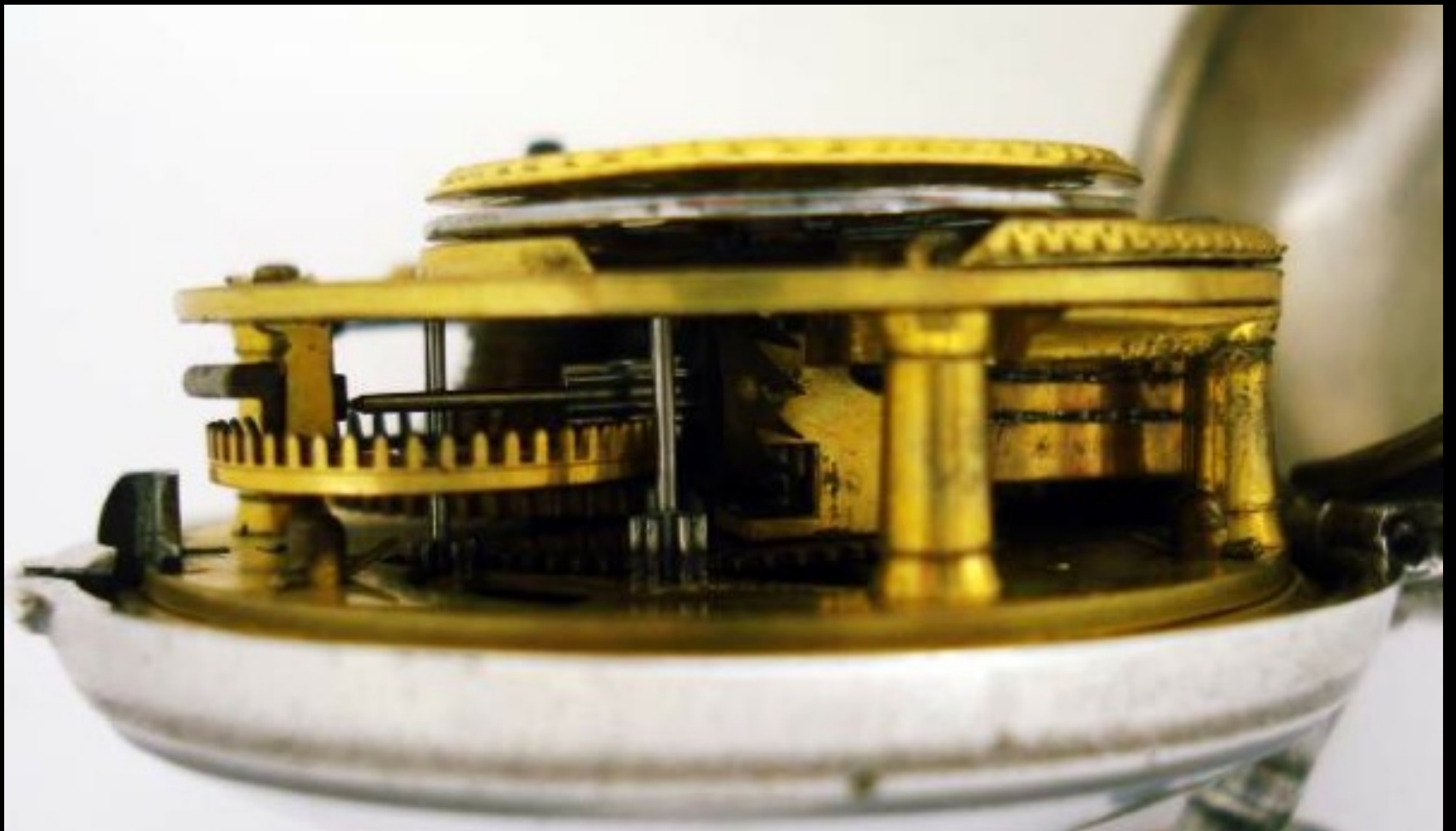
English Silver Repousse Pair Cased Watch with Verge Movement by Nathaniel Sidebottom of Houghton Green 1782 (Cogs & Pieces, Antique Pocket Watches)
