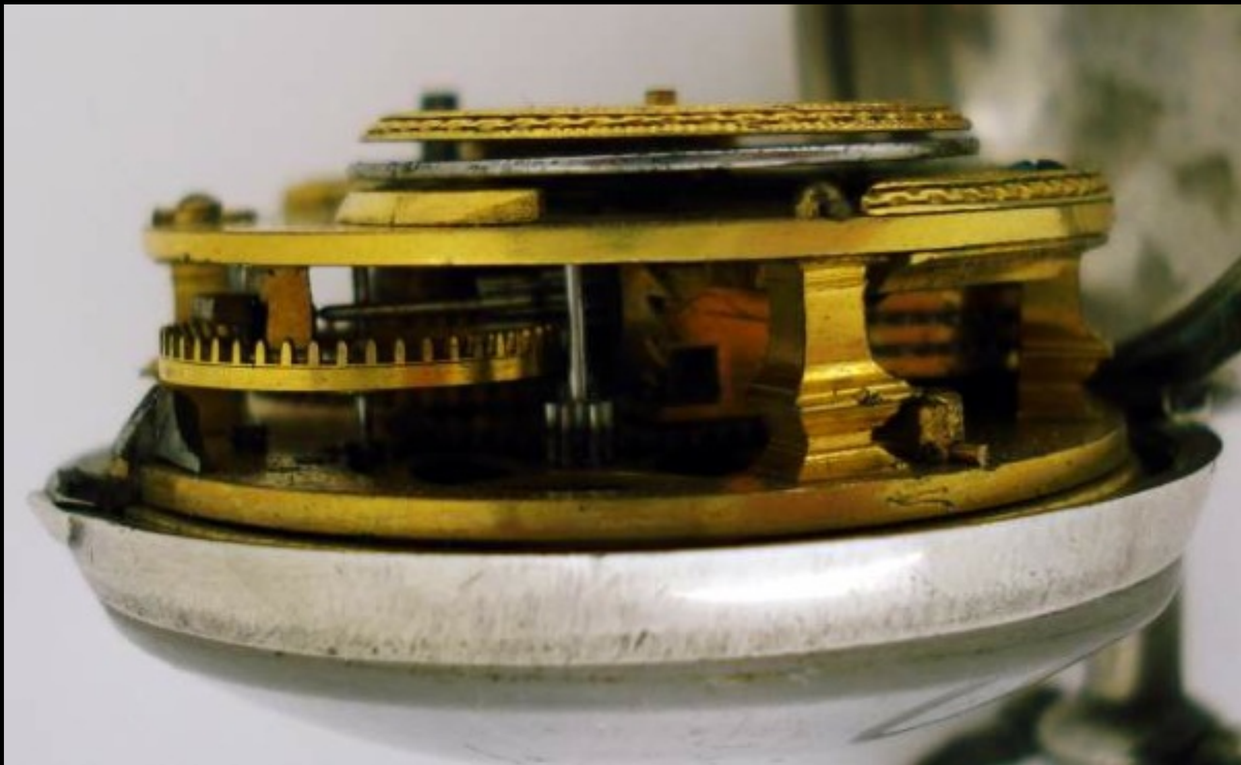
English Silver Pair Cased Watch with Verge Movement by William Bushman of London 1775 (Cogs & Pieces, Antique Pocket Watches)
