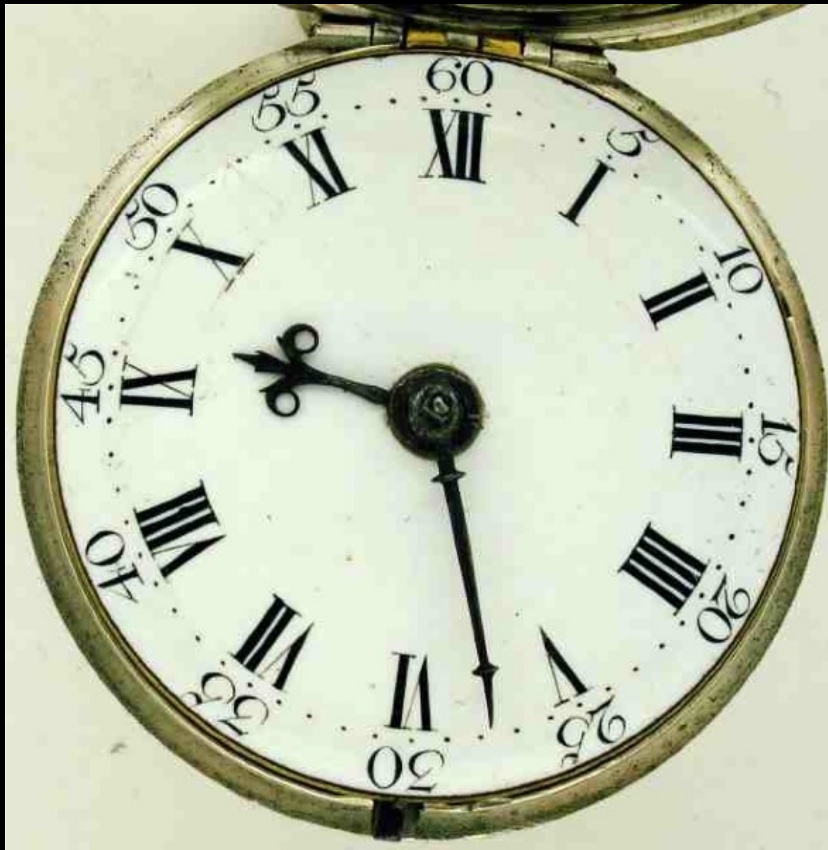
English Silver Pair Cased Watch with Verge Movement by John Purdew of London 1773 (Cogs & Pieces, Antique Pocket Watches)
