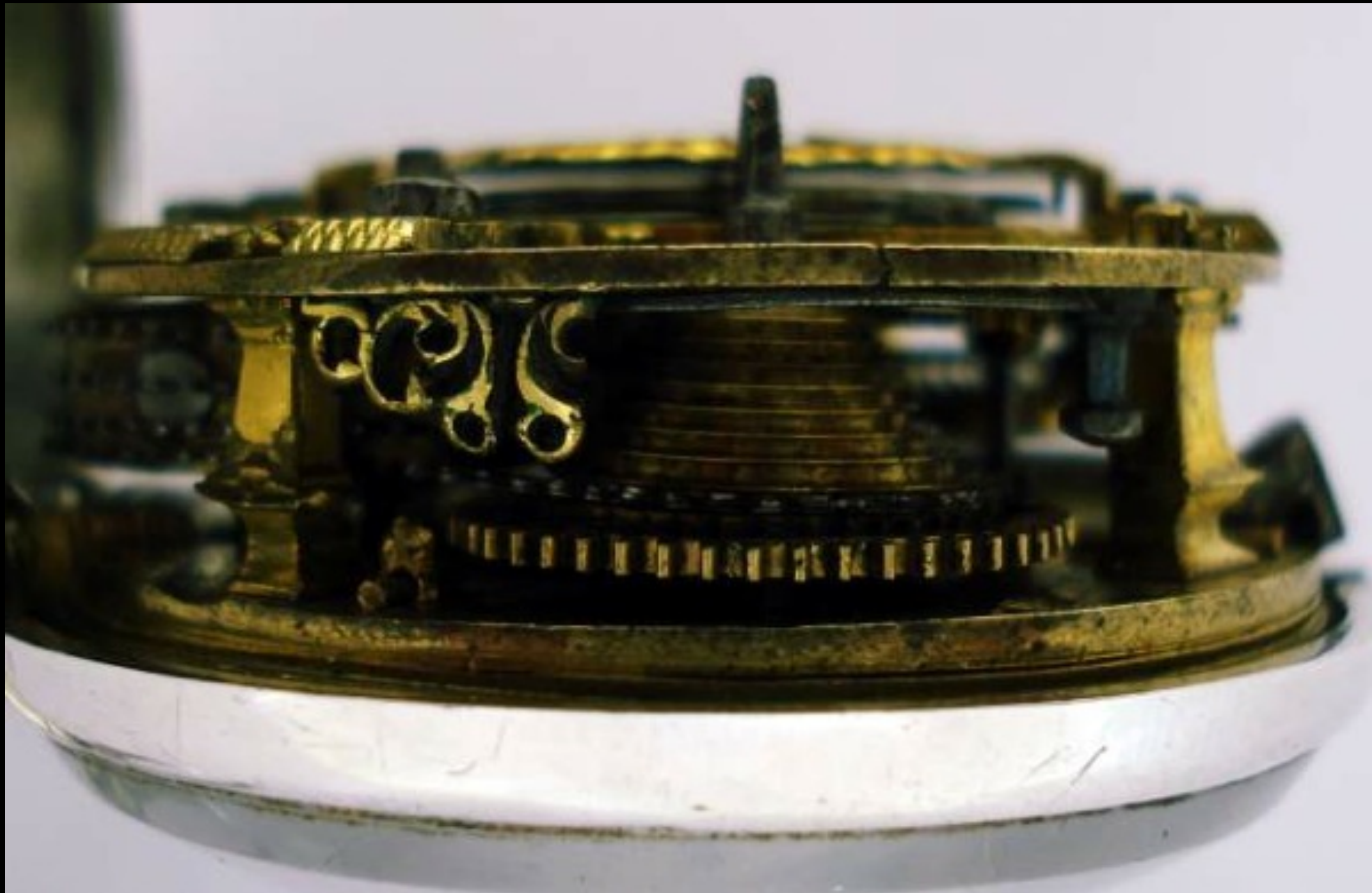
English Silver & Shell Triple Cased Watch with Verge Movement by J. May of London c. 1780 (Cogs & Pieces, Antique Pocket Watches)
