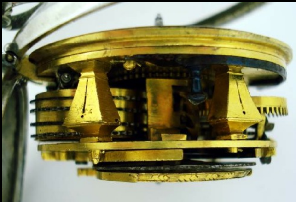
English Silver Pair Cased Watch with Verge Movement by Thomas West of London c. 1690 (Cogs & Pieces, Antique Pocket Watches)
