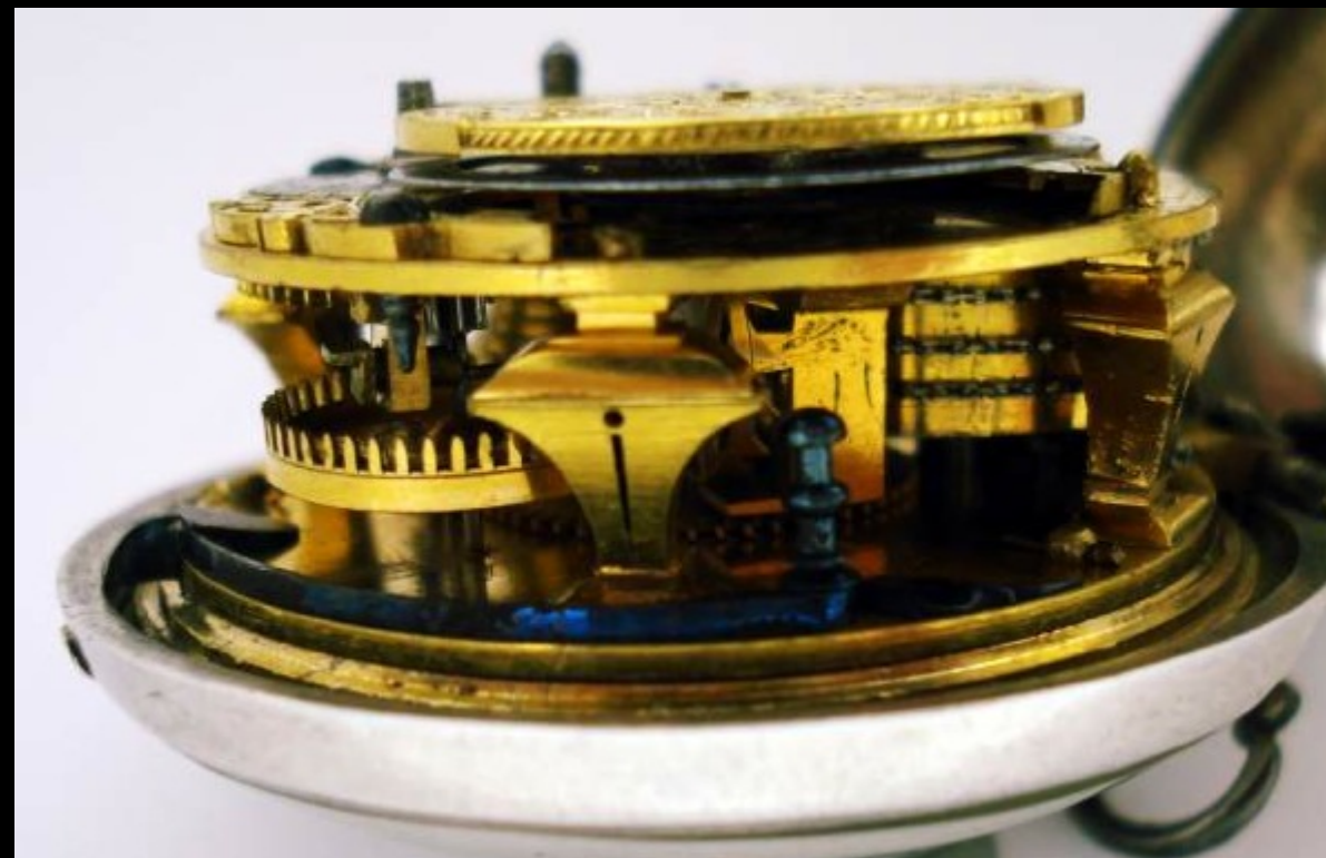
English Silver Pair Cased Watch with Verge Movement by Joseph Foster of London c. 1700 (Cogs & Pieces, Antique Pocket Watches)
