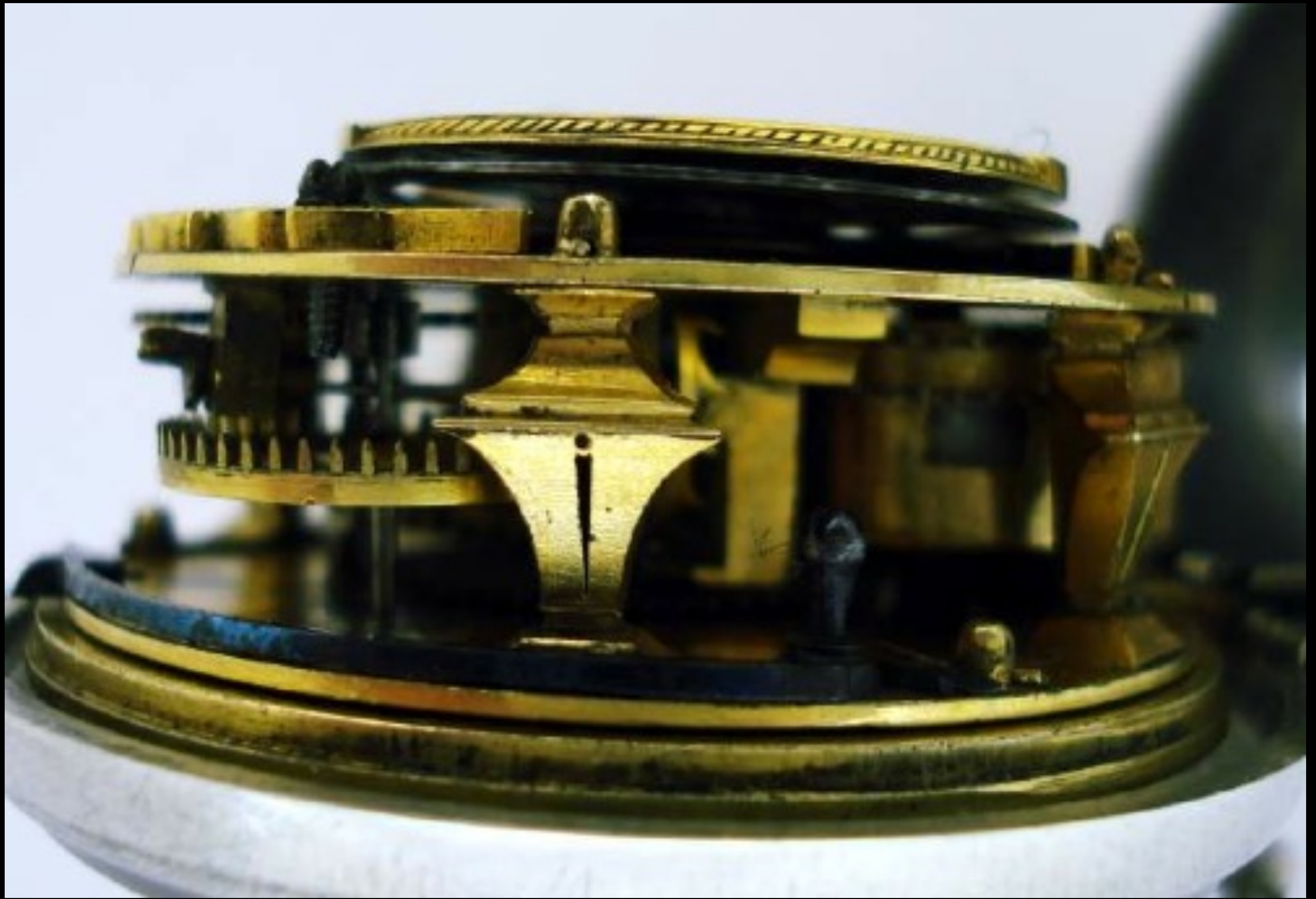
English Silver Pair Cased Watch with Verge Movement by Luke Wise of Reading c. 1700 (Cogs & Pieces, Antique Pocket Watches)
