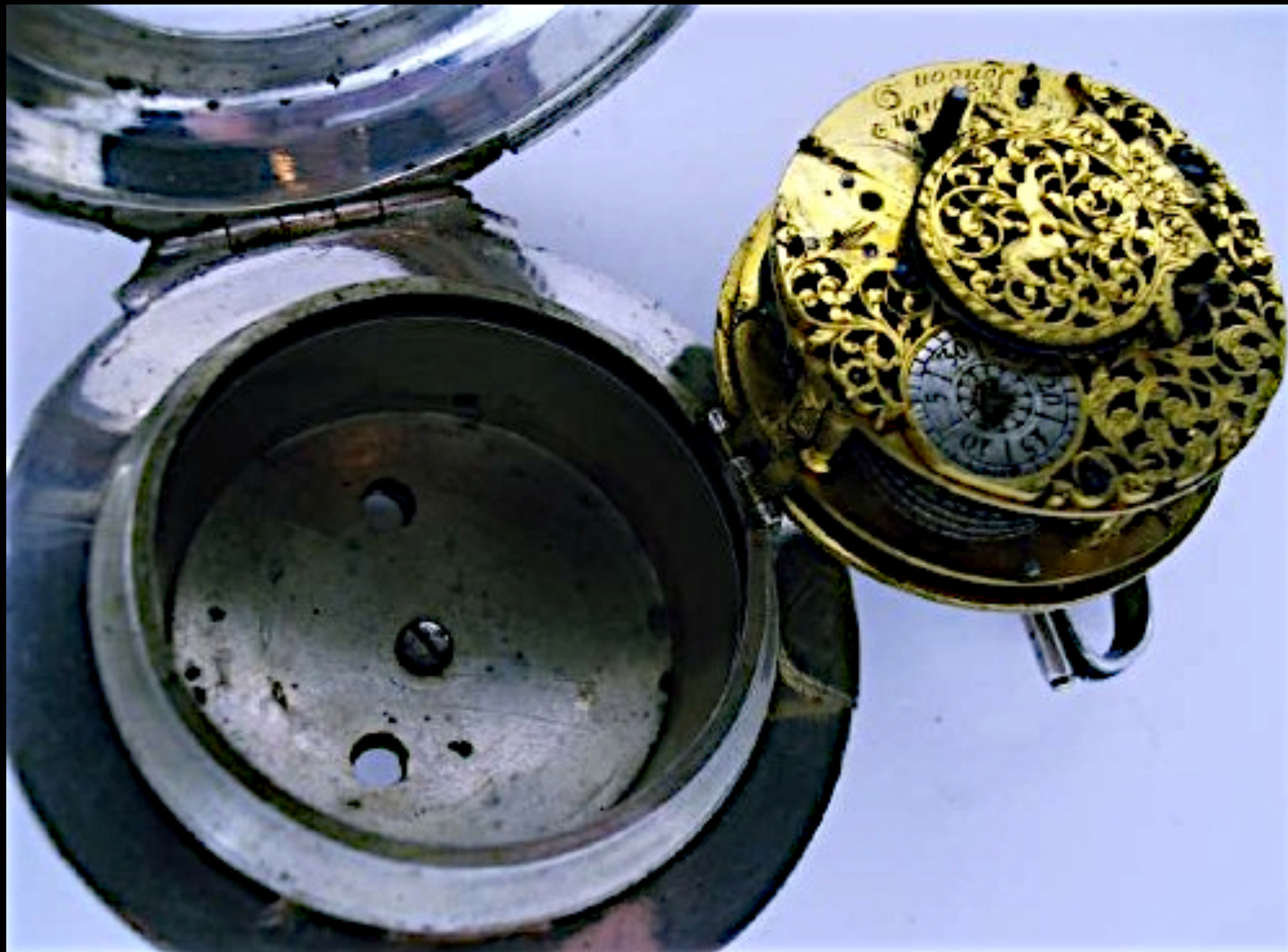
English Silver & Shell Pair Cased Watch with Verge Movement by Tompion of London c. 1690 (Cogs & Pieces, Antique Pocket Watches)
