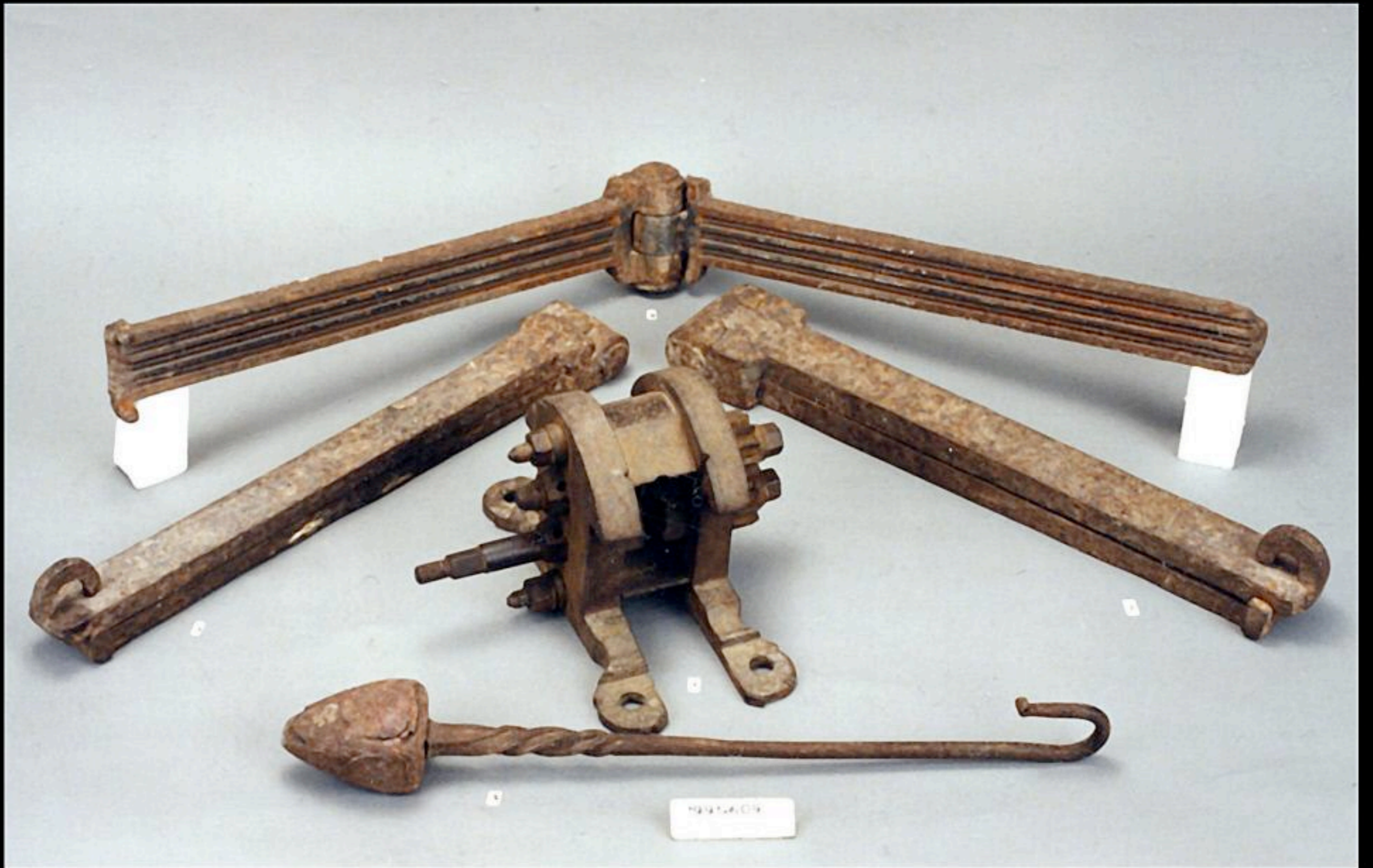
English Glazier's Rolling Mill for Lead Window Comes Used to Assemble Leaded Casement Windows Dated 1755 (Colonial Williamsburg)
