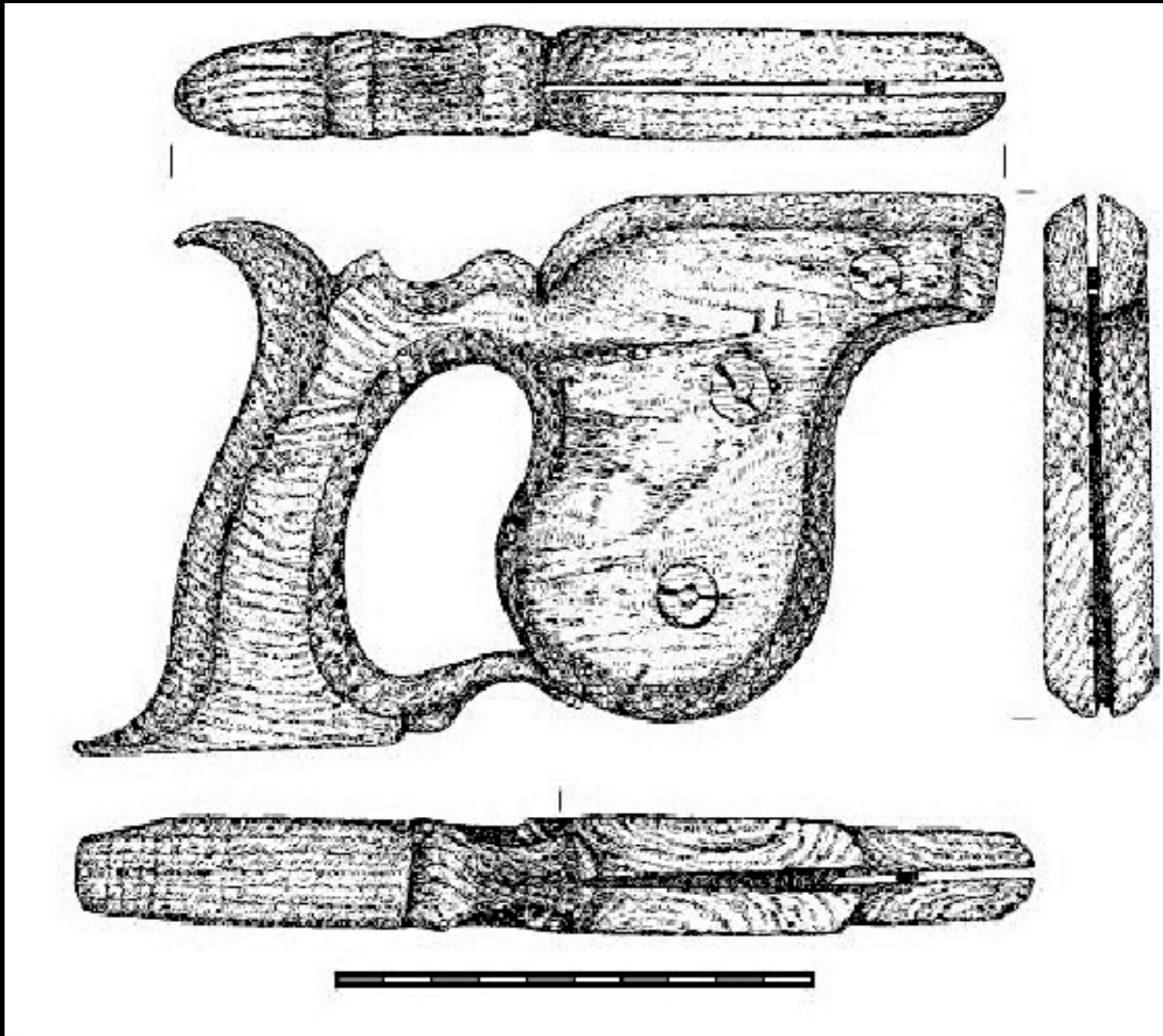
Saw Handle Recovered from the Wreck of the General Carleton of Whitby 1785
